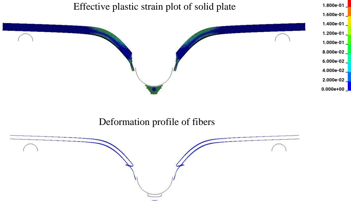
Figure 3. FEM (conforming mesh) results.
