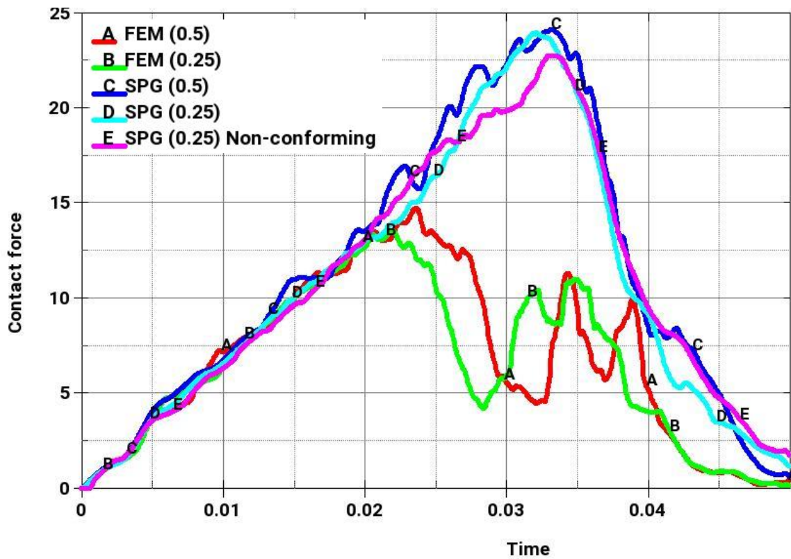
Figure 5. SPG (non-conforming mesh) results.
