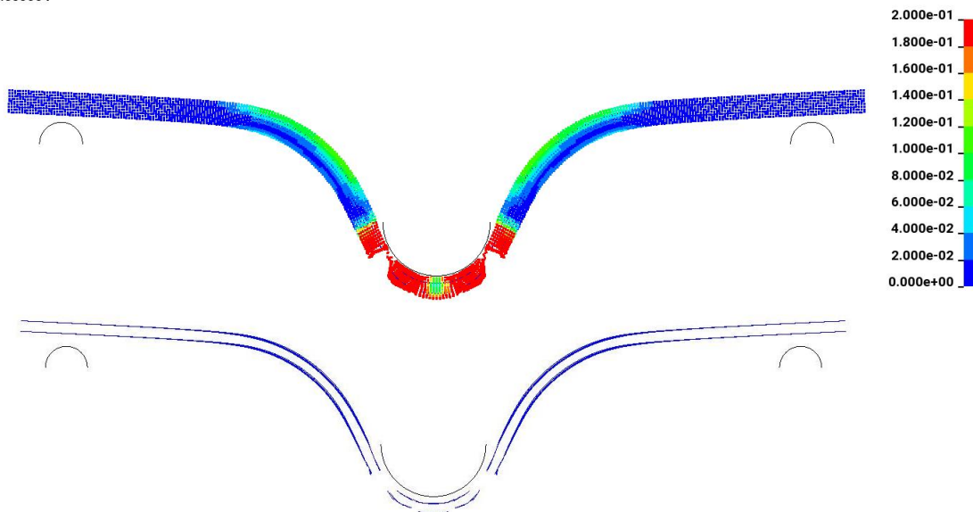
Figure 4. SPG (conforming mesh) results.
